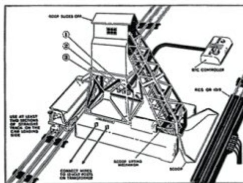
Figure 1—Lionel No. 97 Coal Elevator in Layout showing Transformer and Controller Connections.
